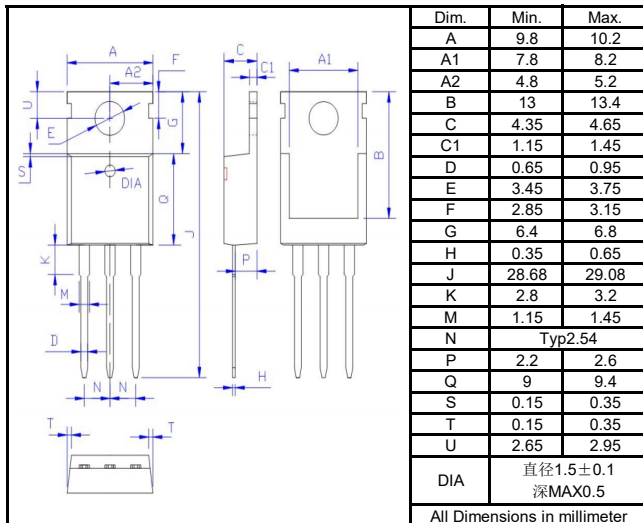
TO-220C
